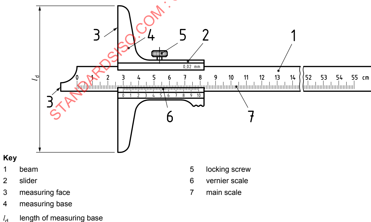
Figure 1 — Example for a design of a calliper depth gauge (slider with locking screw)
