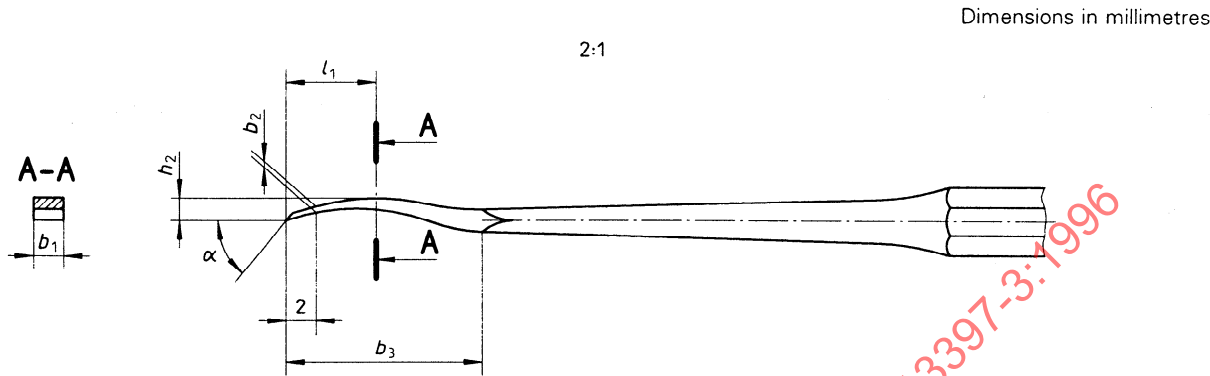
Figure 1 — Dental scalers — H-types 3 and 4 (chisel)
