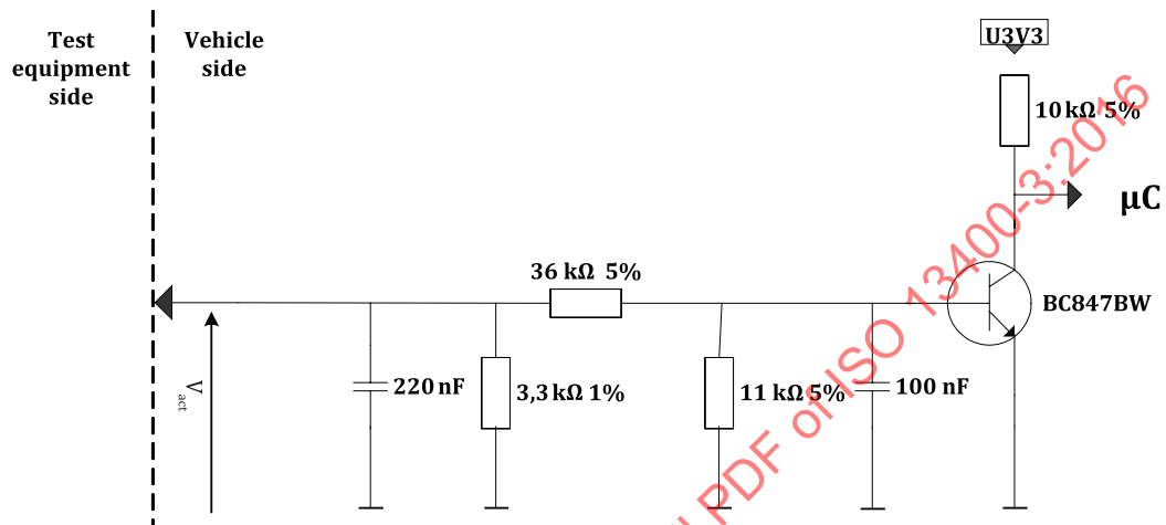
Figure 5 — Activation line circuit example – Option 2
