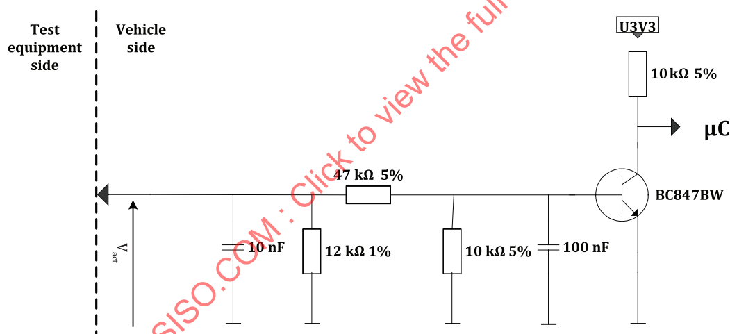
Figure 4 — Activation line circuit example – Option 1
