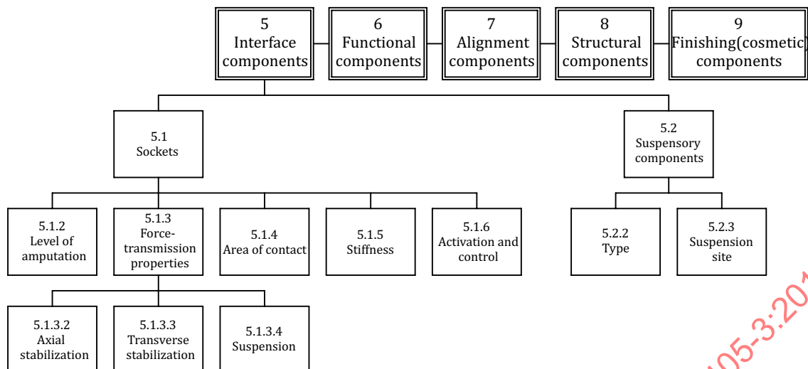
Figure 1 — Upper limb prosthetic components — Classification tree
