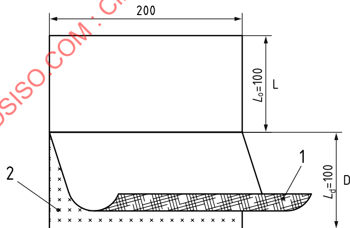
Figure 3 — Dimensions of a shear test specimen
