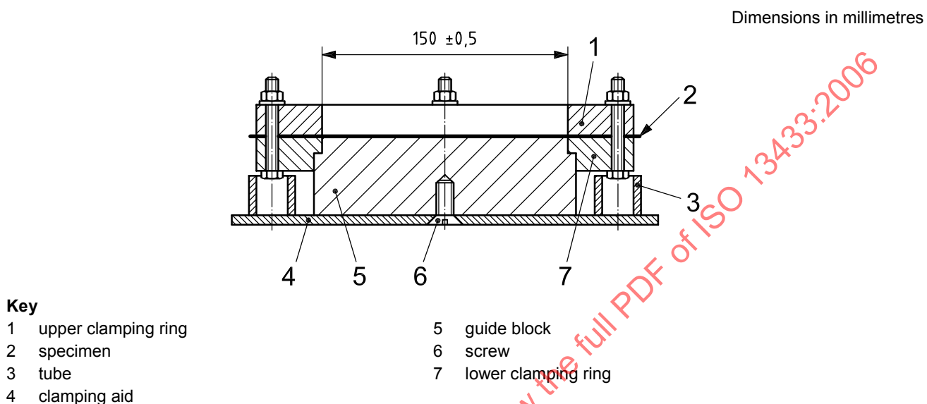
a) Example of clamping rings, guide block use
