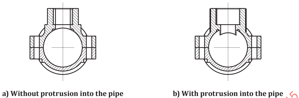
Figure 1 — Examples of plastics saddles
