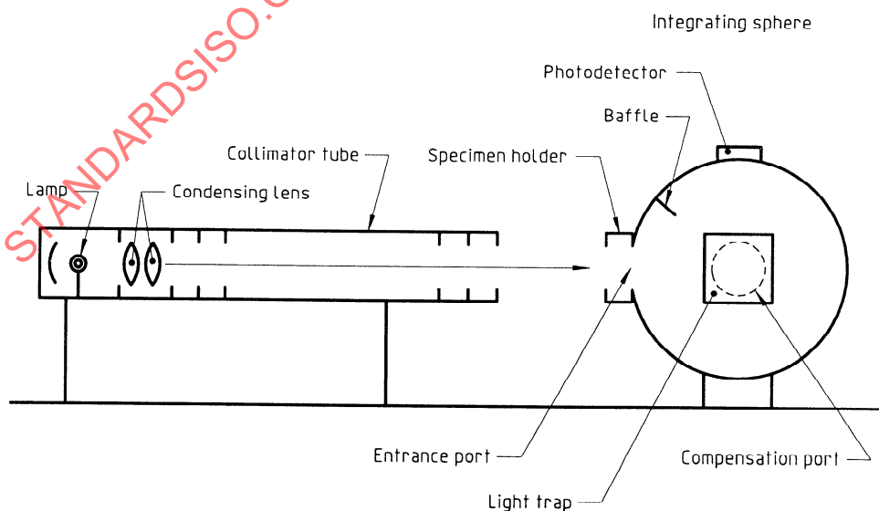
Figure 1 — Schematic arrangement of the apparatus
