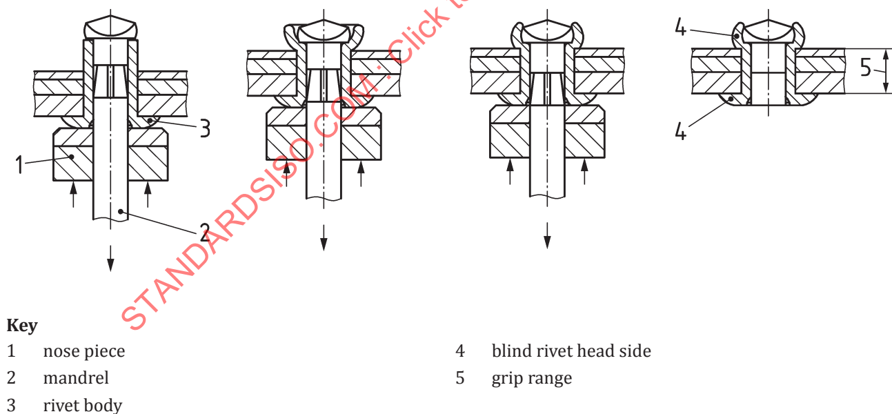
Figure A.1 — Blind rivet setting sequence illustration
