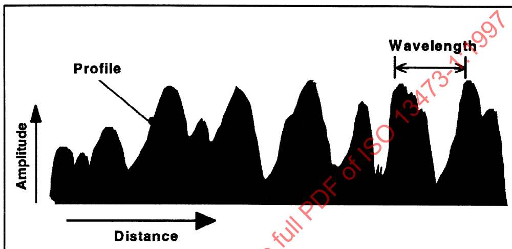
Figure A.1 — Illustration of some basic terms describing pavement surface characteristics
