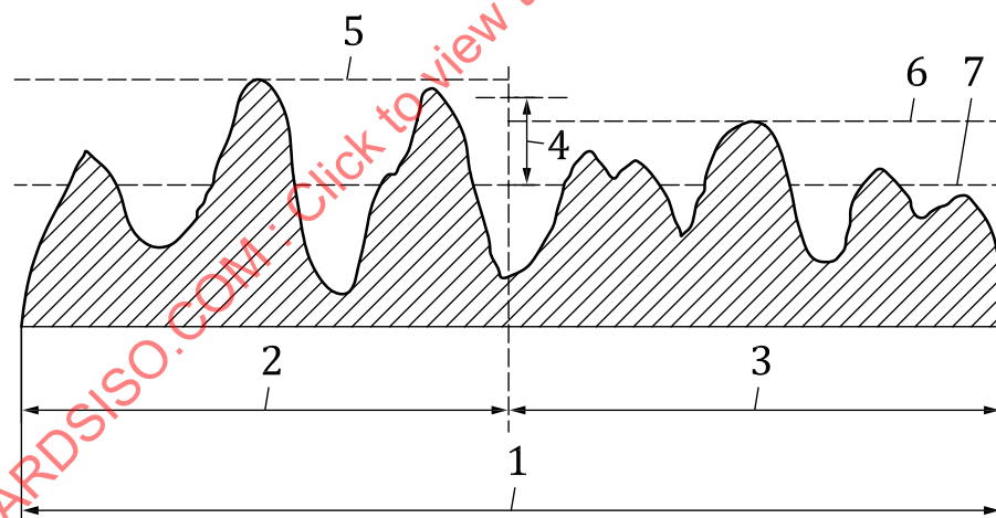
Figure A.3 — Illustration of the terms “surface” and “TD”
