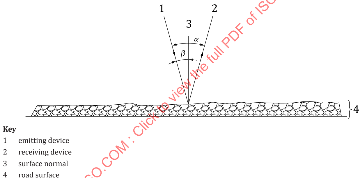
Figure 1 — Requirements regarding alignment of non-contact sensors above a road surface
