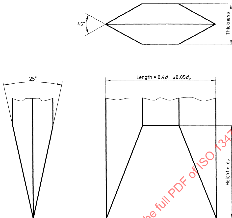
Figure 2 — Striker-blade geometry
