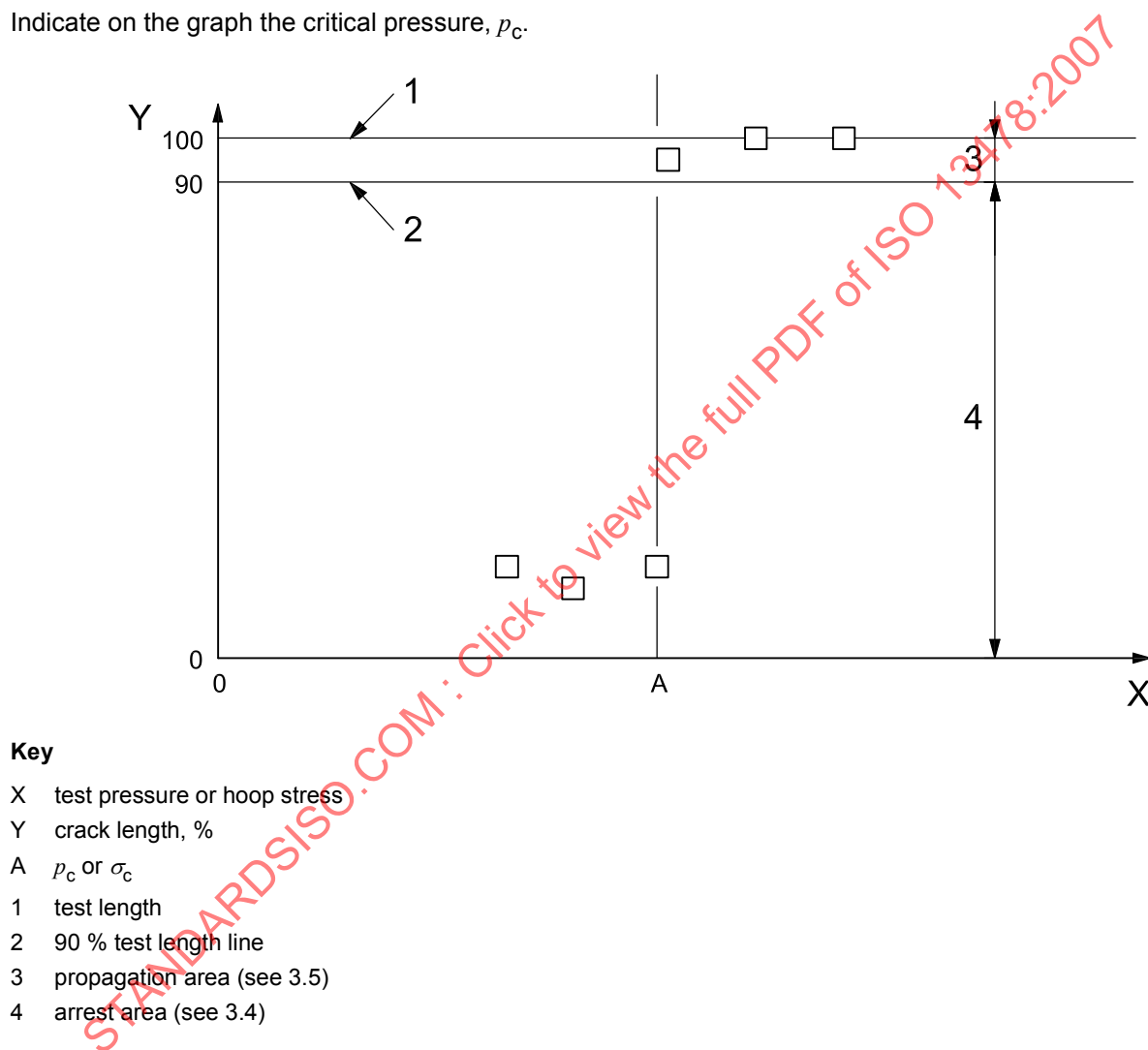
Figure A.1 — Typical test-data plot to determine the critical pressure ( p_c ) or critical hoop stress ( \sigma_c )
