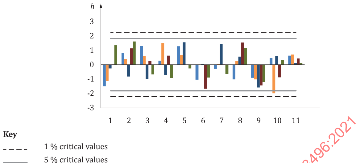
Figure E.5 — Amaranth content — Mandel's interlaboratory consistency statistic, h , grouped by laboratories
