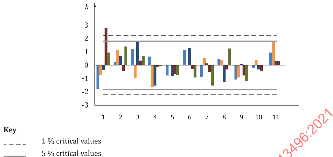
Figure E.15 — Brilliant Blue FCF content — Mandel's interlaboratory consistency statistic, h , grouped by laboratories
