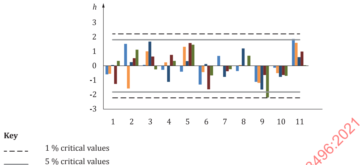
Figure E.9 — Ponceau 4R content — Mandel's interlaboratory consistency statistic, h , grouped by laboratories
