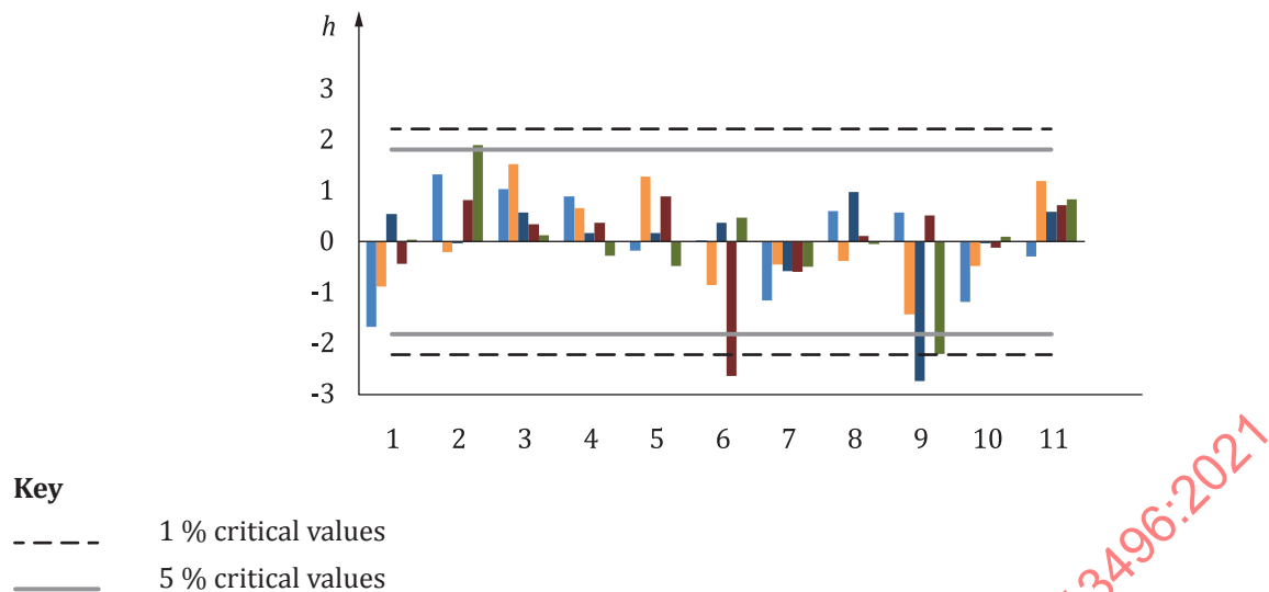
Figure E.7 — Indigotine content — Mandel's interlaboratory consistency statistic, h , grouped by laboratories
