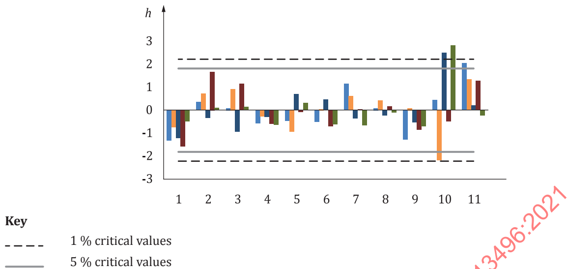
Figure E.1 — Tartrazine content — Mandel's interlaboratory consistency statistic, h , grouped by laboratories
