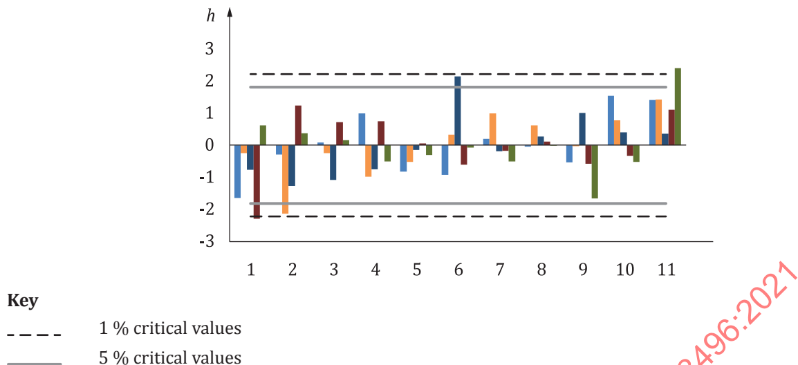
Figure E.13 — Allura Red AC content — Mandel's interlaboratory consistency statistic, h , grouped by laboratories
