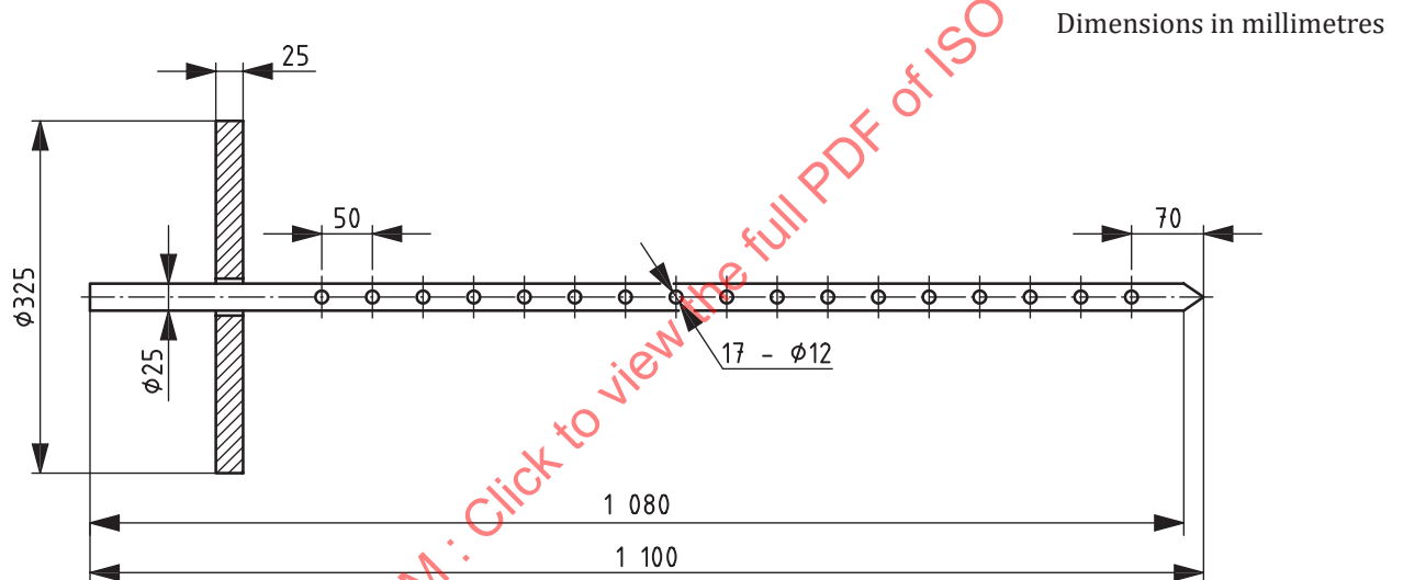
Figure 1 — Stand sampling device
