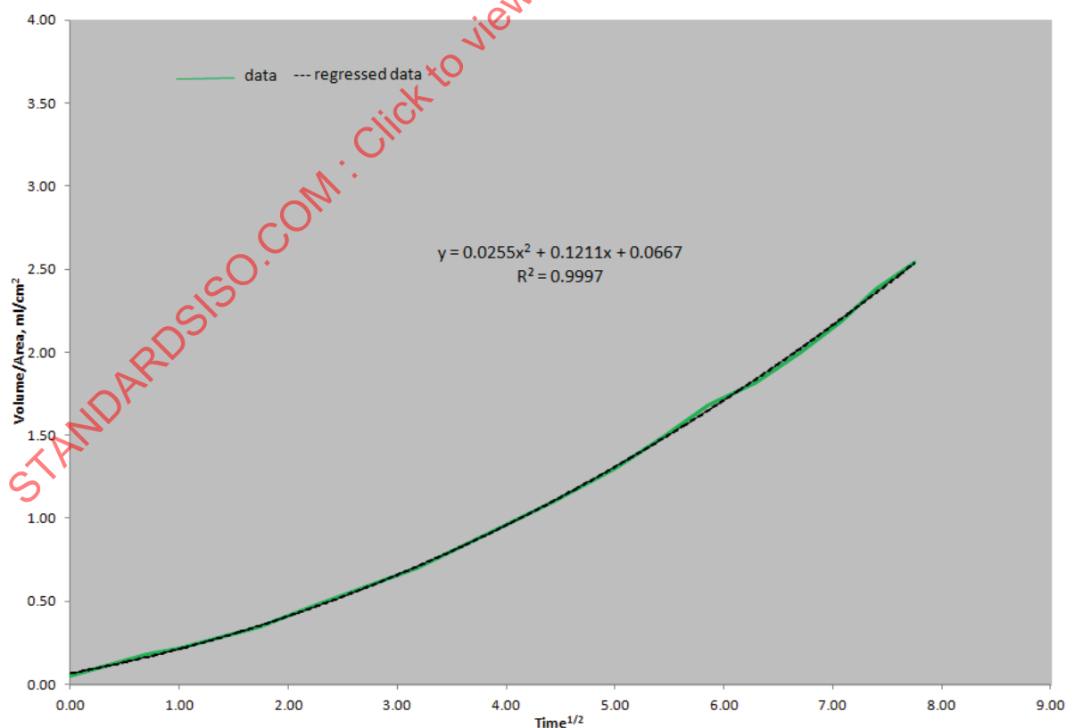
Figure 5 — Dynamic fluid loss example — 4,2 kg/m 3 (35 lb/Mgal) Zr/CMHPG, at 93 °C (200 °F), 6 900 kPa (1 000 psi)
