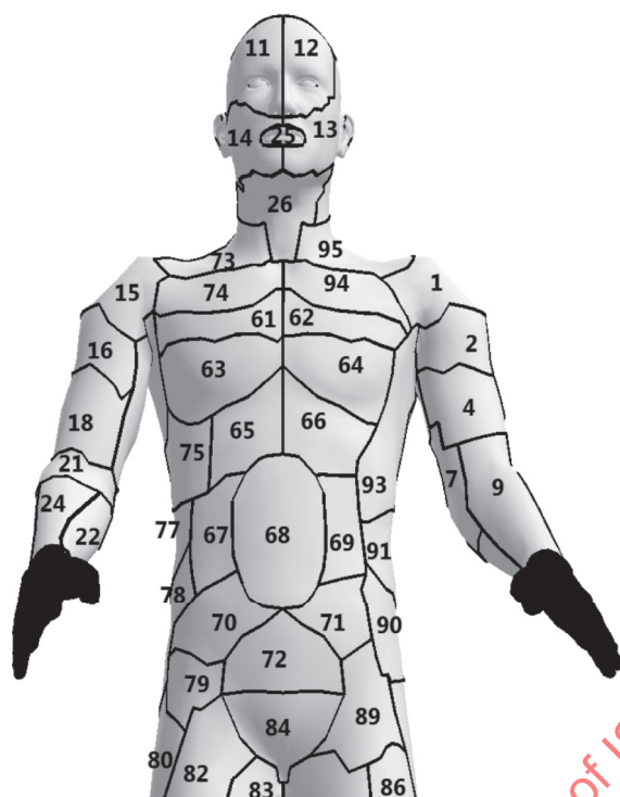
Figure 5 — Example of manikin sensor location and their associated area
