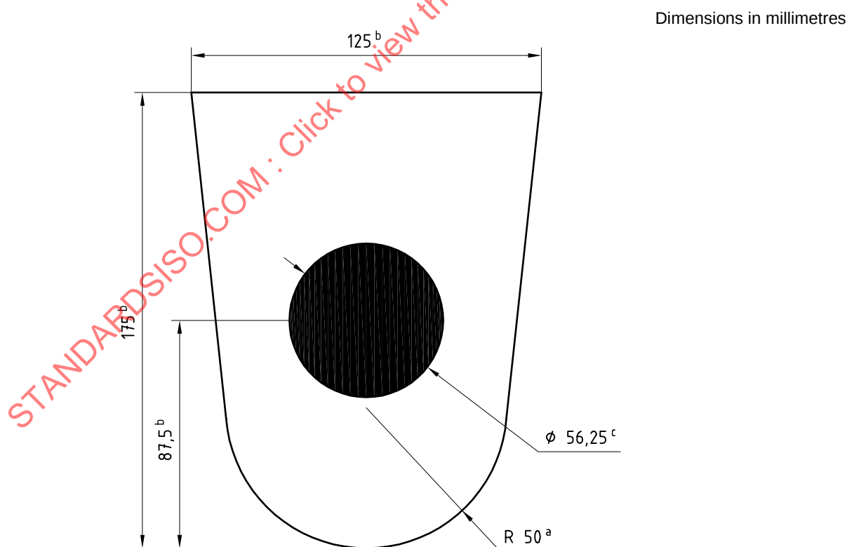
Figure 4 — Equivalent-round models — Complex shapes
