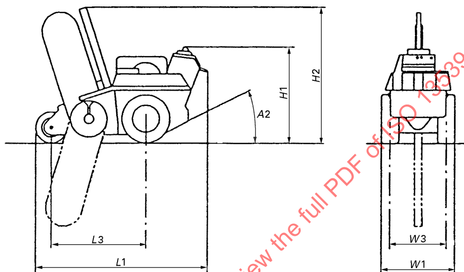
Figure 1 — Pedestrian-operated trencher
