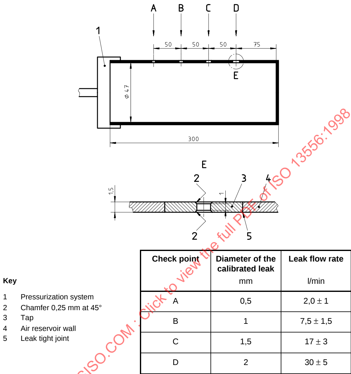
Figure 5 — Verification system for the ultrasonic equipment
