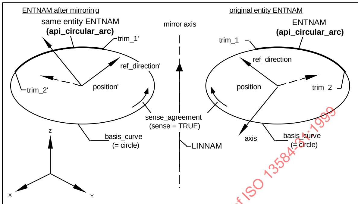
Figure A. 50 — Function: Mirror_Ent (3D view)
