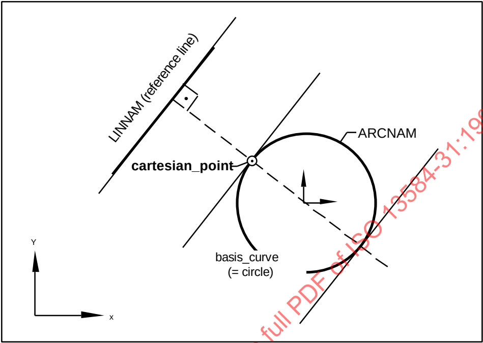
Figure A.13 — Function: Pnt_Tangential_Arc
