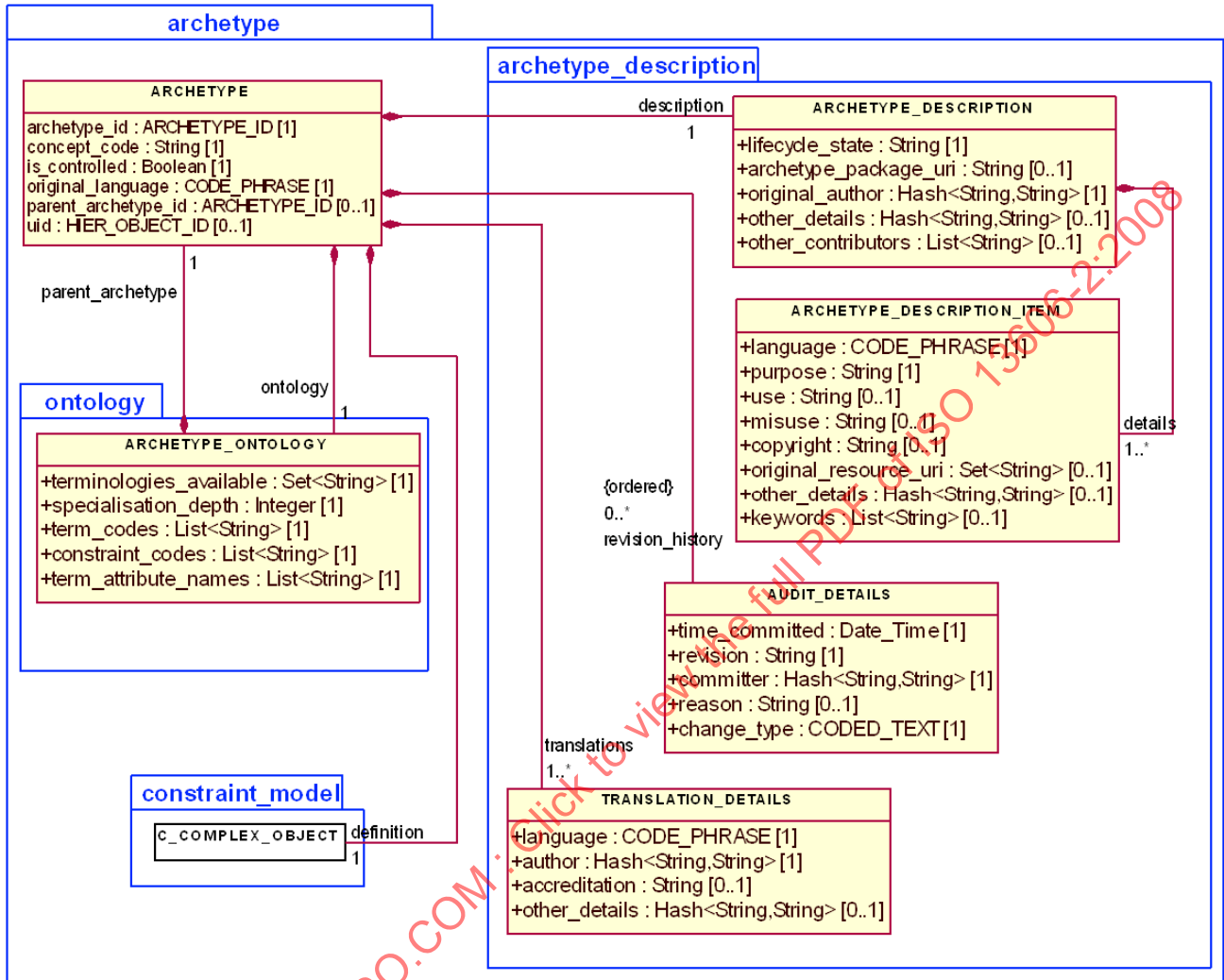
Figure 5 — Archetype package
