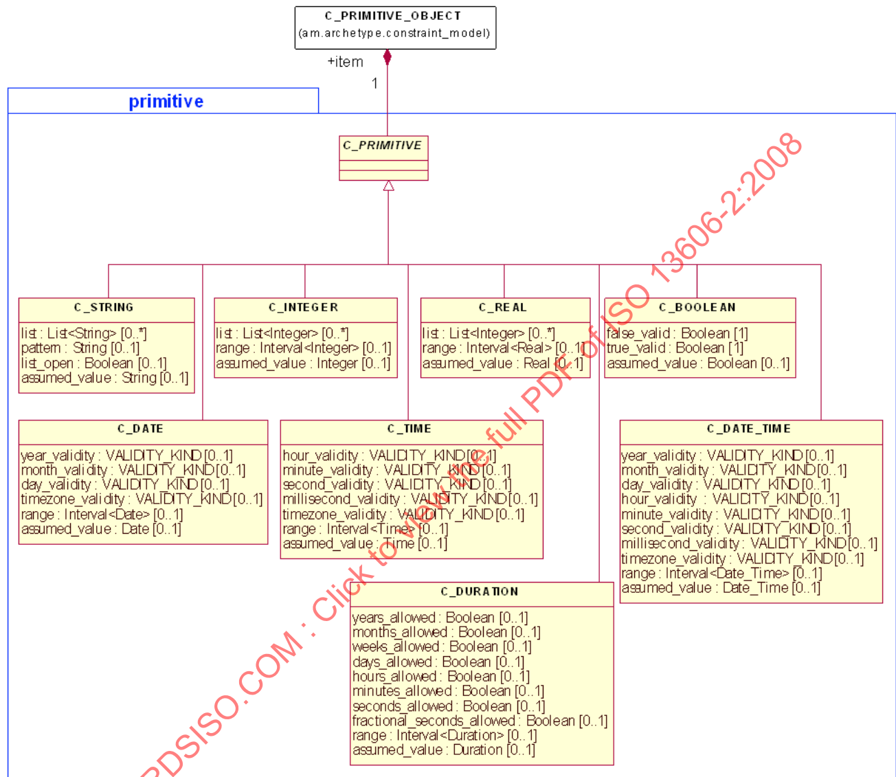
Figure 9 — Primitive package
