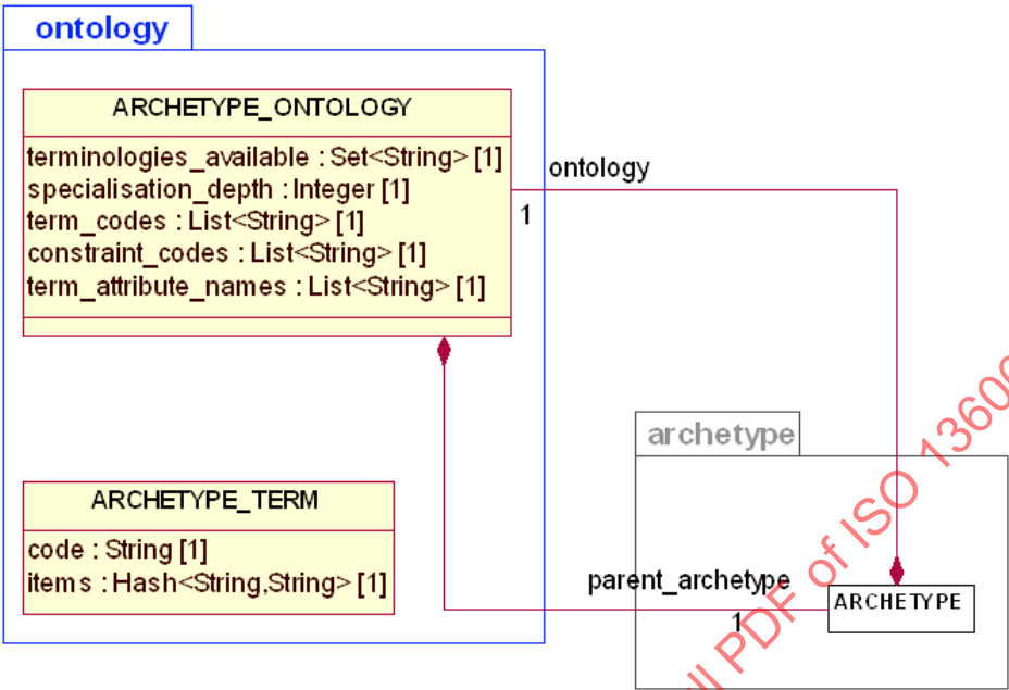
Figure 10 — Ontology package
