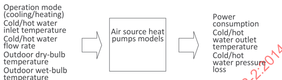
Figure D.6 — Inputs and outputs of air-cooled heat pumps models
