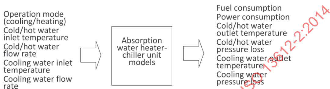
Figure D.4 — Inputs and outputs of absorption water heater-chiller unit models
