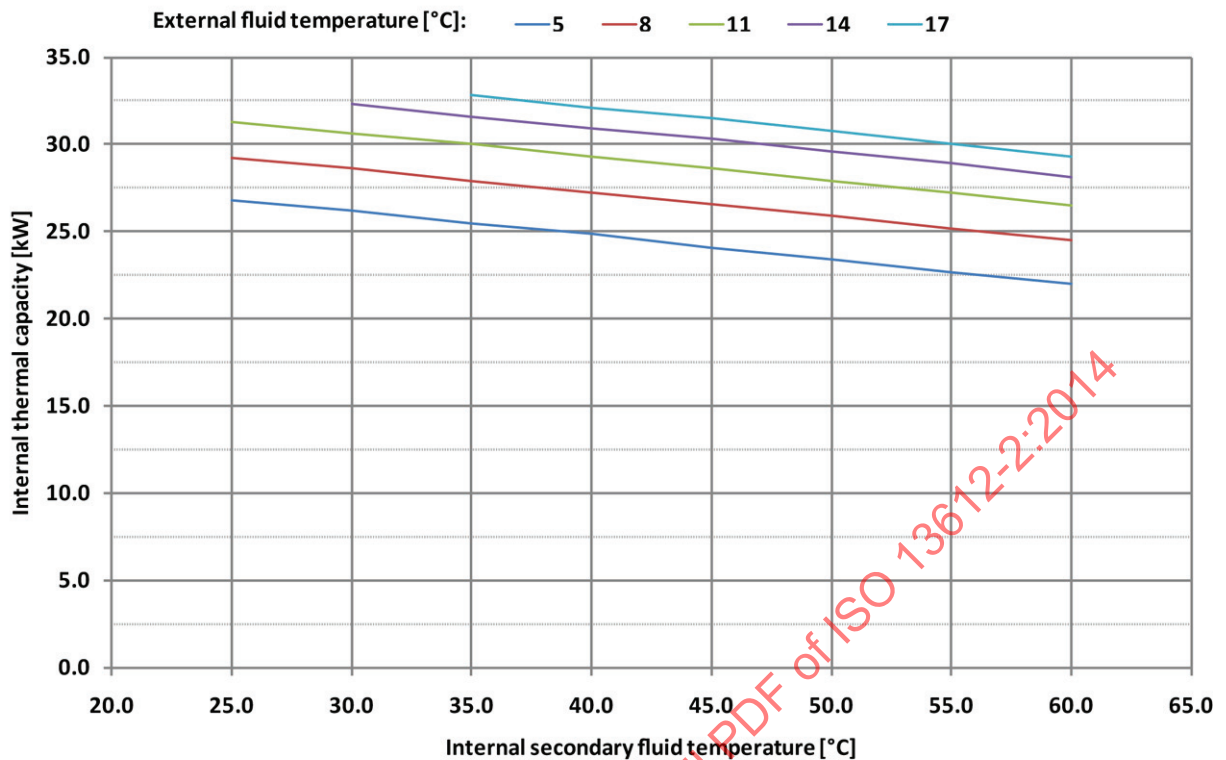
b) Thermal capacity at the internal side versus external and internal secondary fluid temperatures (heating mode)
