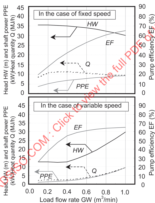
Figure D.14 — Characteristics of pump models (examples of rated flow rate of 1 m³/min)
