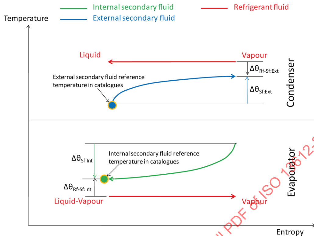
b) Cooling case
