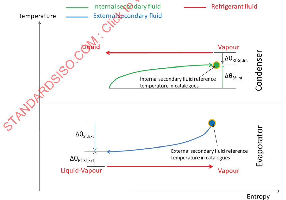
a) Heating case
