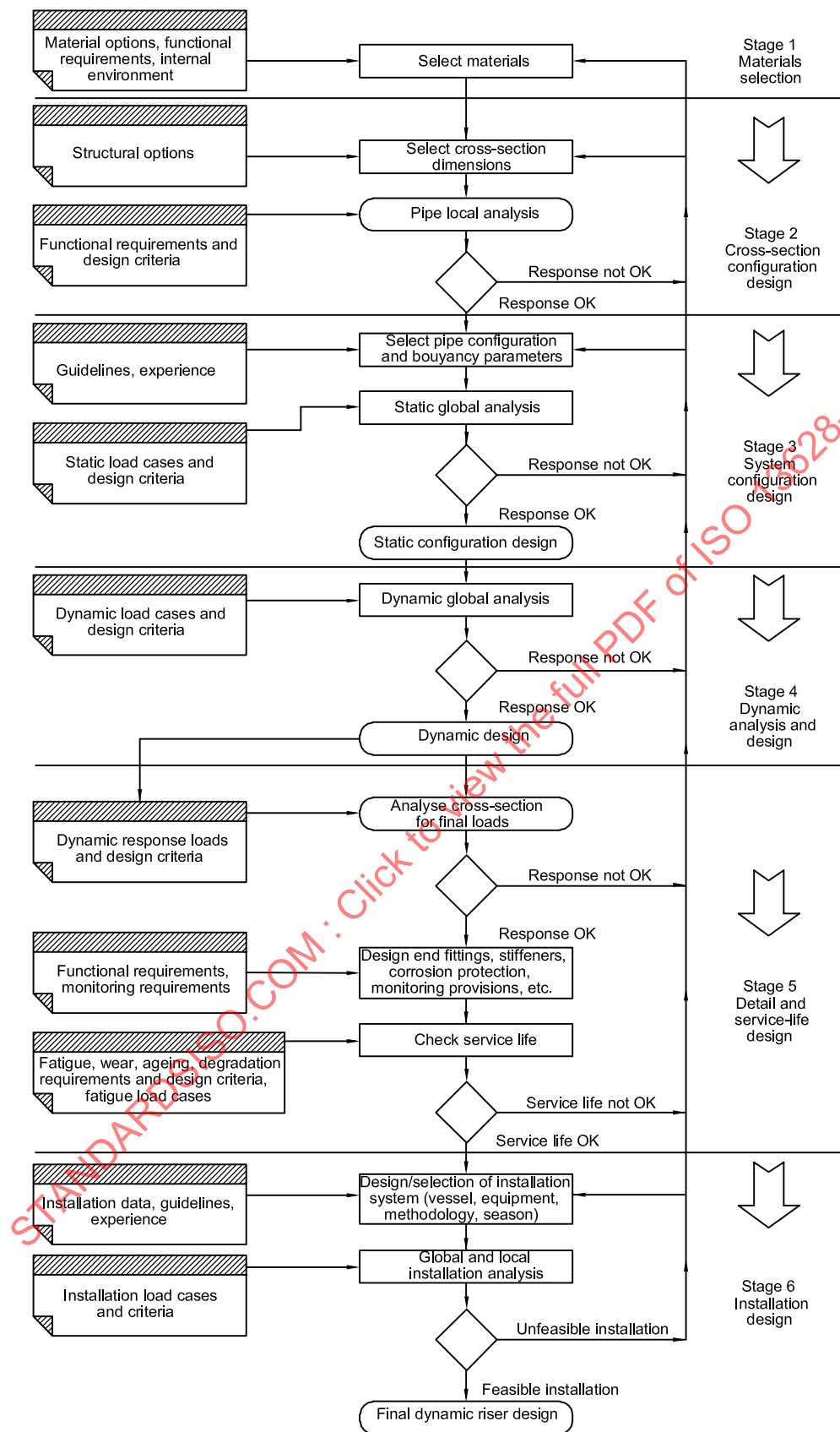
Figure 20 — Dynamic-application design flowchart
