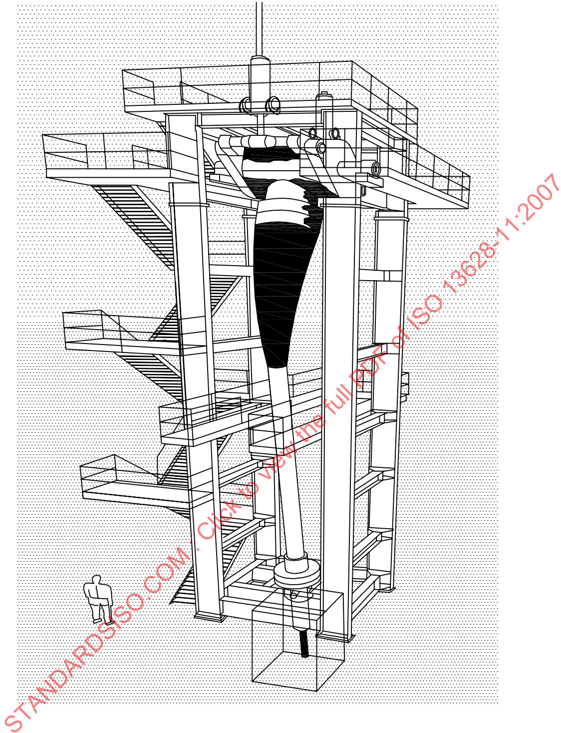
Figure 28 — Typical set-up for a dynamic fatigue test
