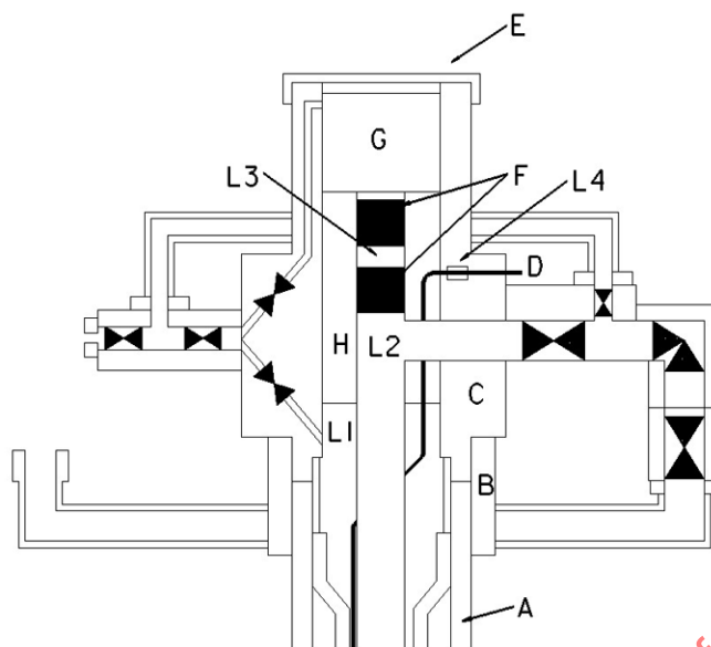
c) Horizontal subsea tree without separate internal tree cap
