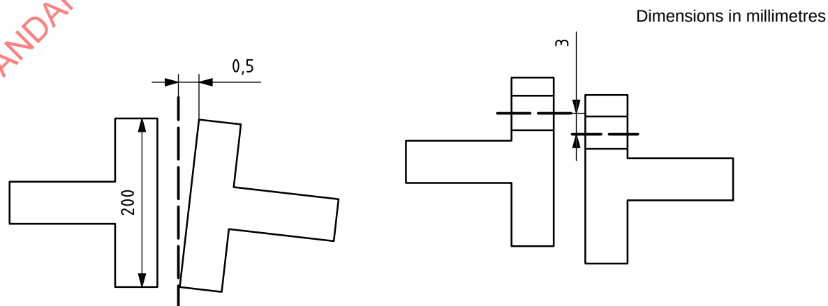
Figure G.1 — Flange-to-flange alignment tolerances
