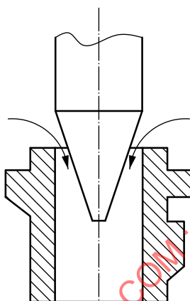
b) Needle and seat
