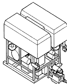
d) Single-point docking tool delivery system
