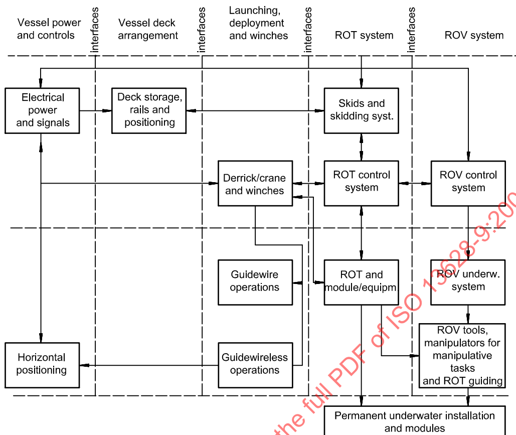
Figure 3 — Illustration of interfaces between the intervention vessel, the ROT system and, when used, the ROV system
