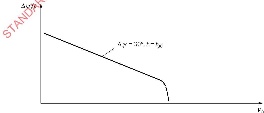
Figure 4 — Mean turning rate vs. ship speed
