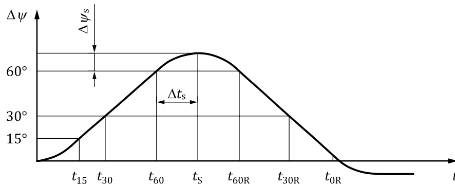
Figure 3 — Test at zero speed
