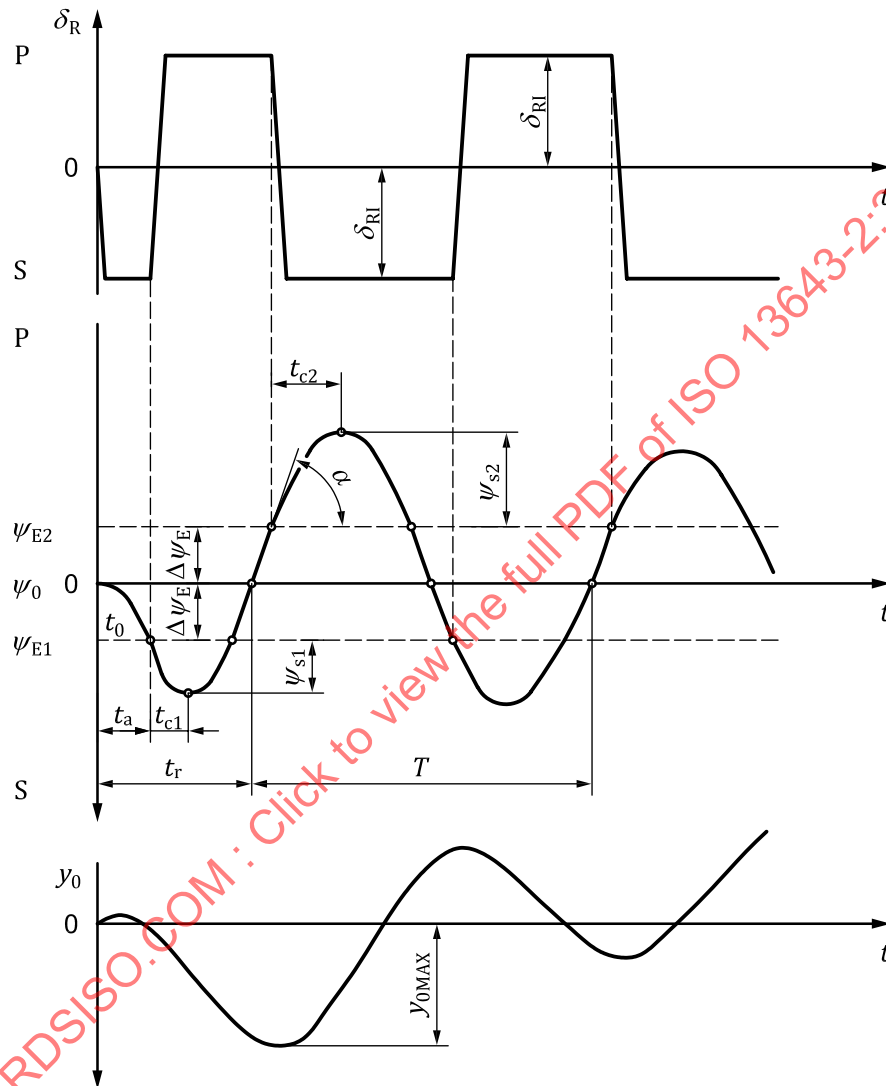
Figure 5 — Time histories of the zig-zag test
