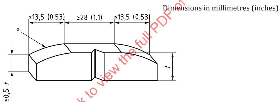
Figure B.5 — Orientation of impact test pieces
