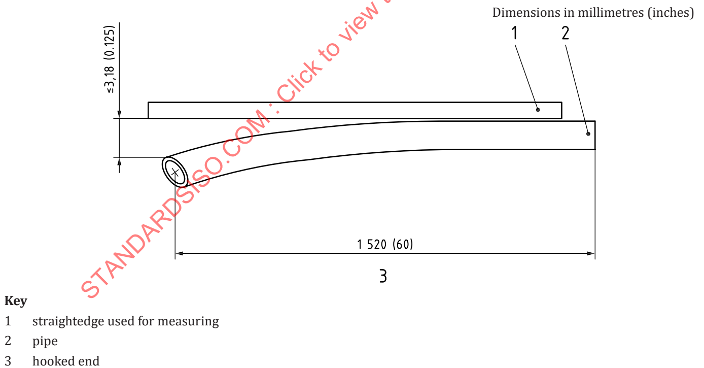
Figure B.2 — Measuring end straightness
