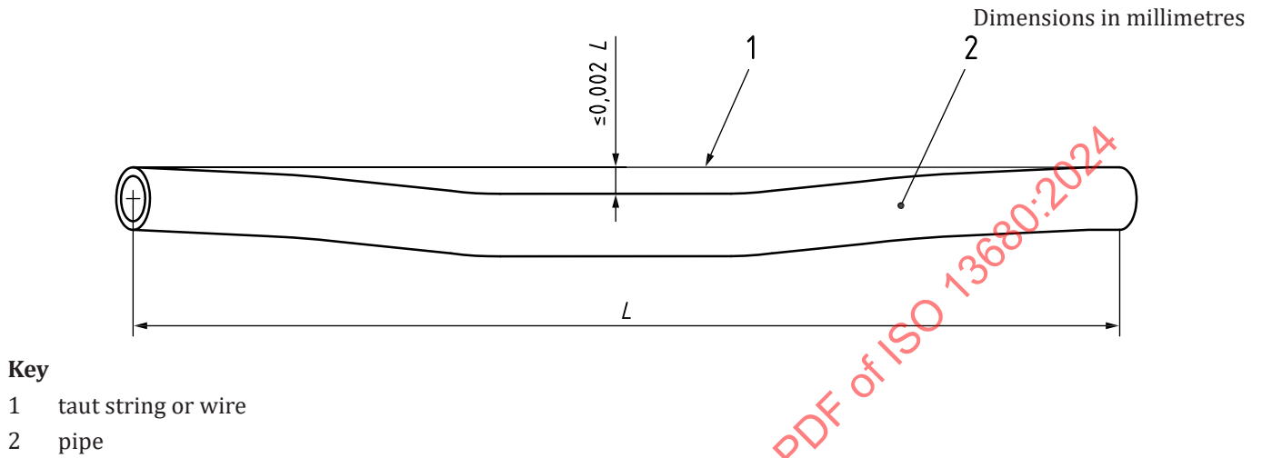
Figure B.1 — Measuring full-length straightness
