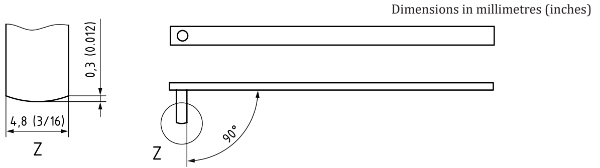
Figure B.3 — Example of a typical 90° hook-type tool
