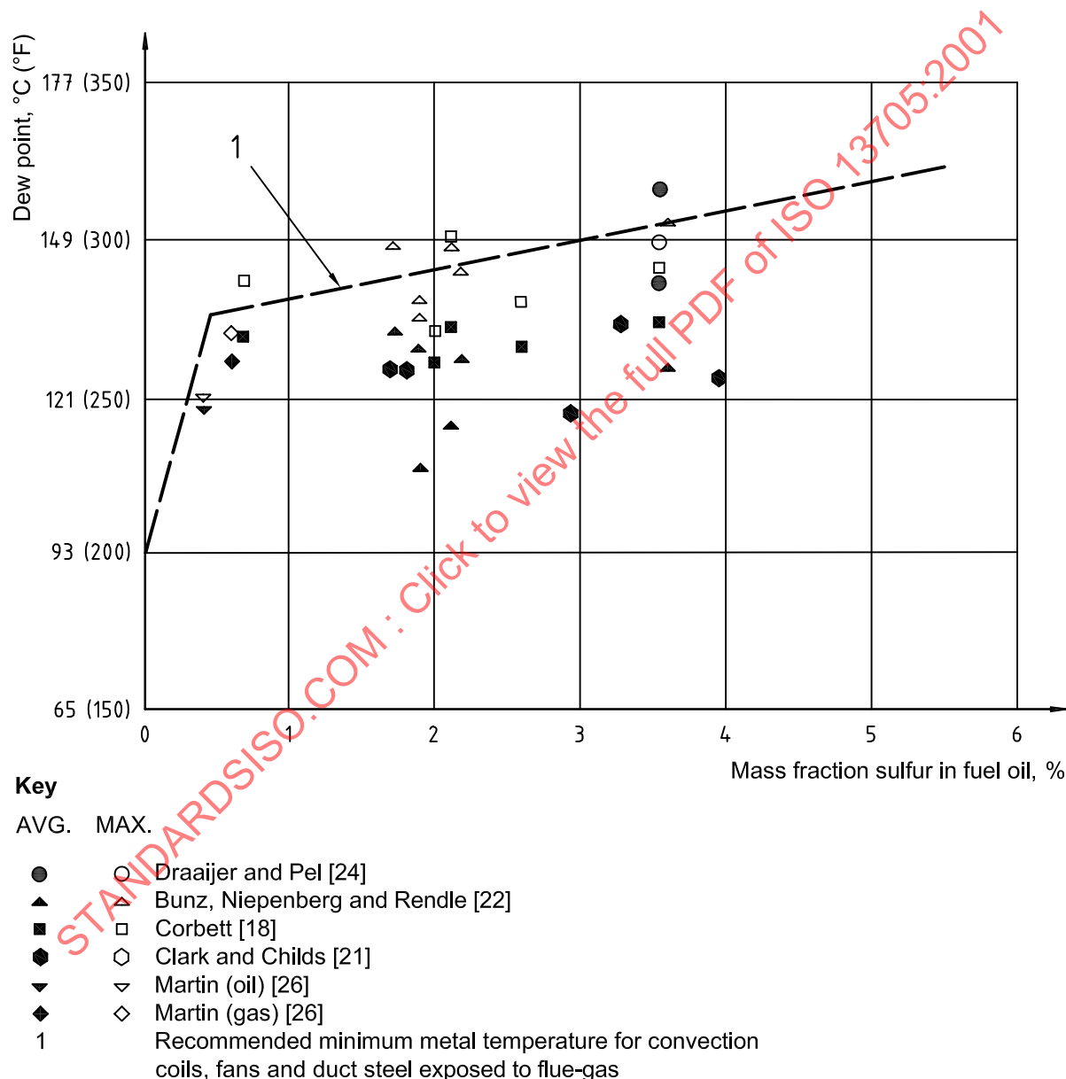
Figure F.8 — Dew points of flue-gas versus sulfur in fuel oil (test data from industrial boilers)
