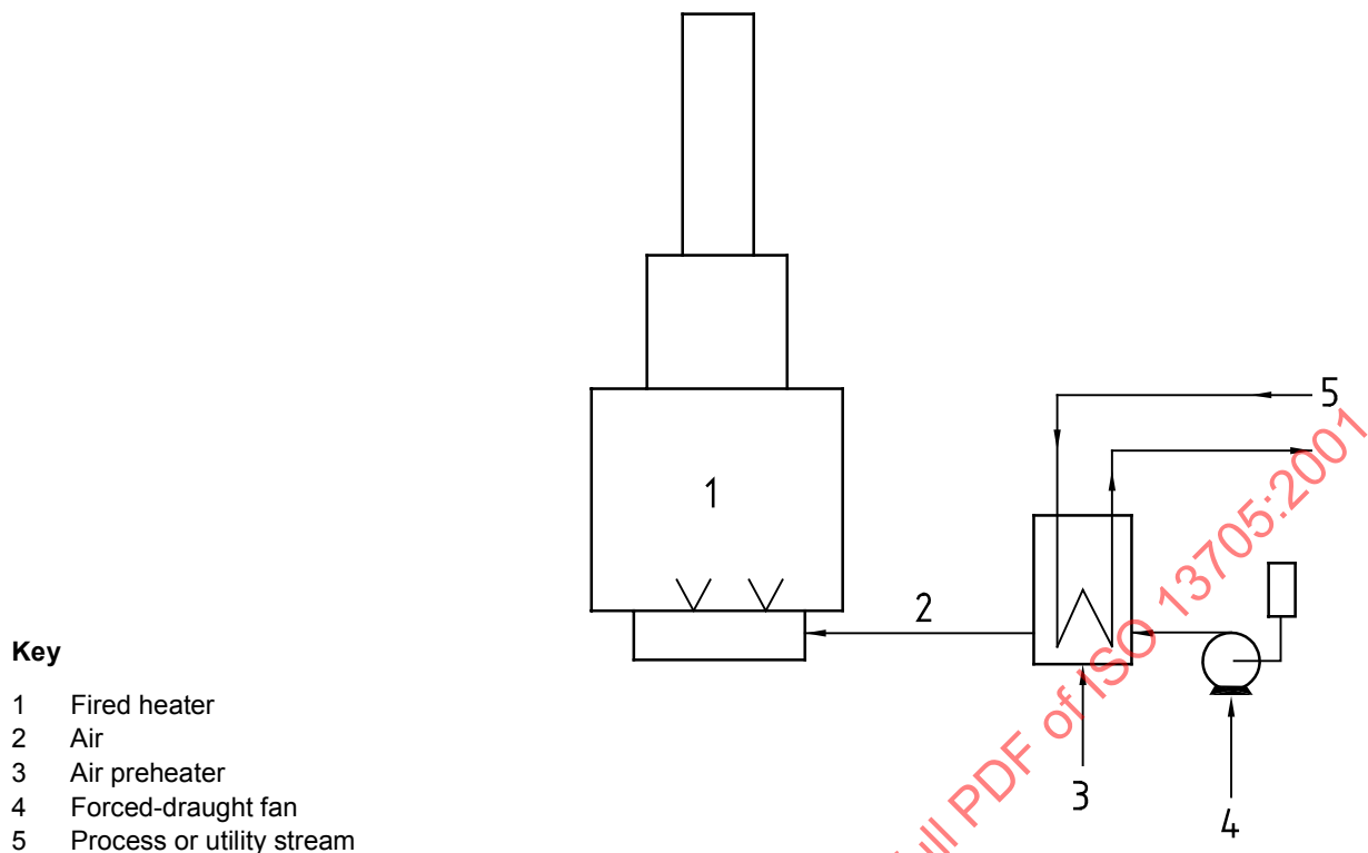
Figure 6 — External heat source for air preheating
