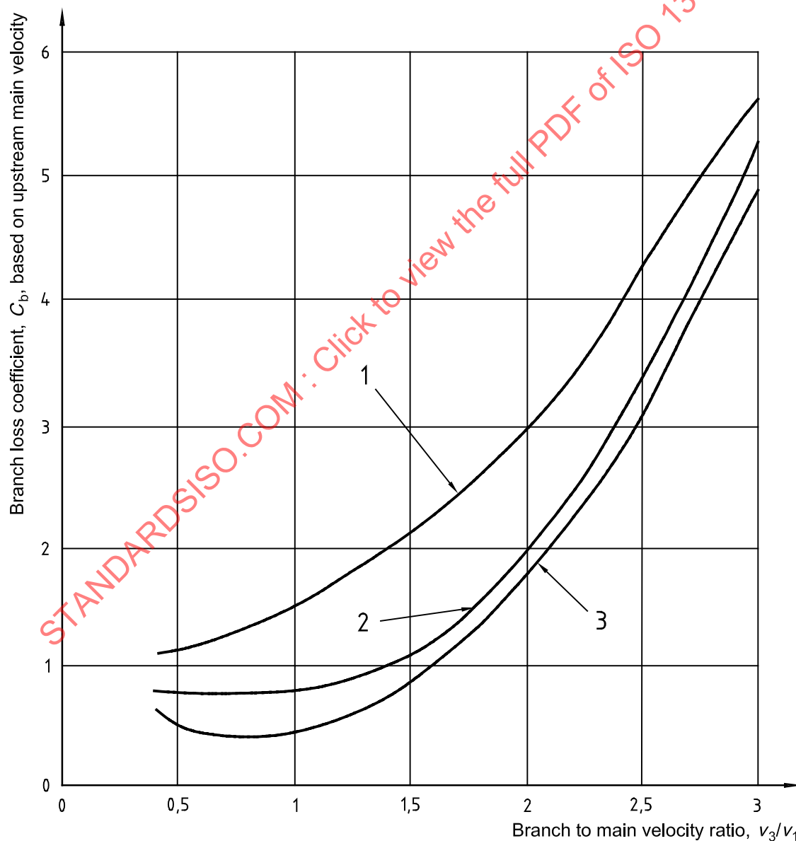
Figure F.6 — Branch loss coefficients
