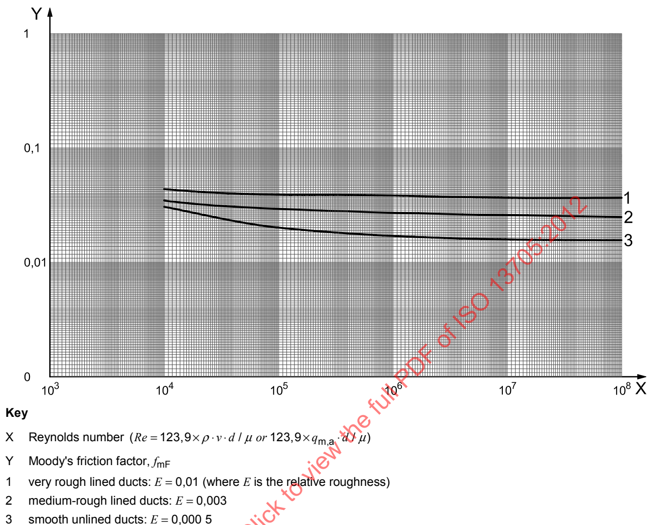
Figure F.7 — Moody's friction factor versus Reynolds number
