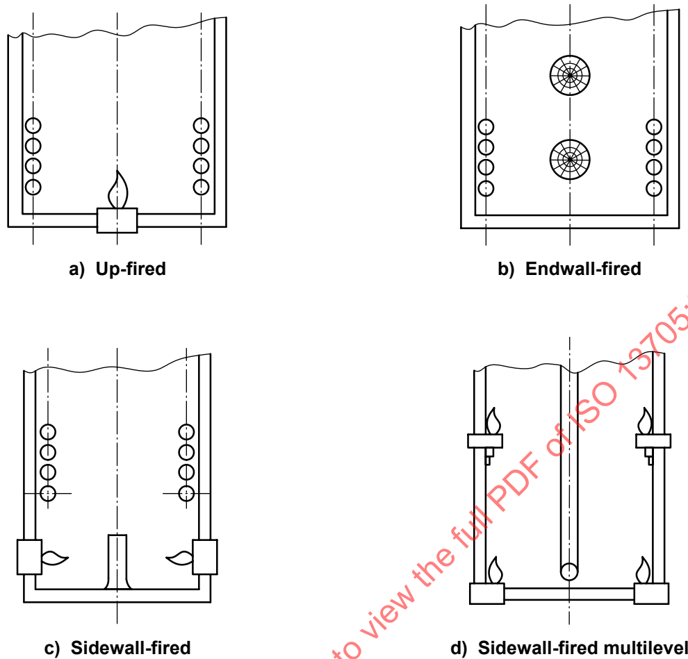
Figure 2 — Typical burner arrangements (elevation view)
