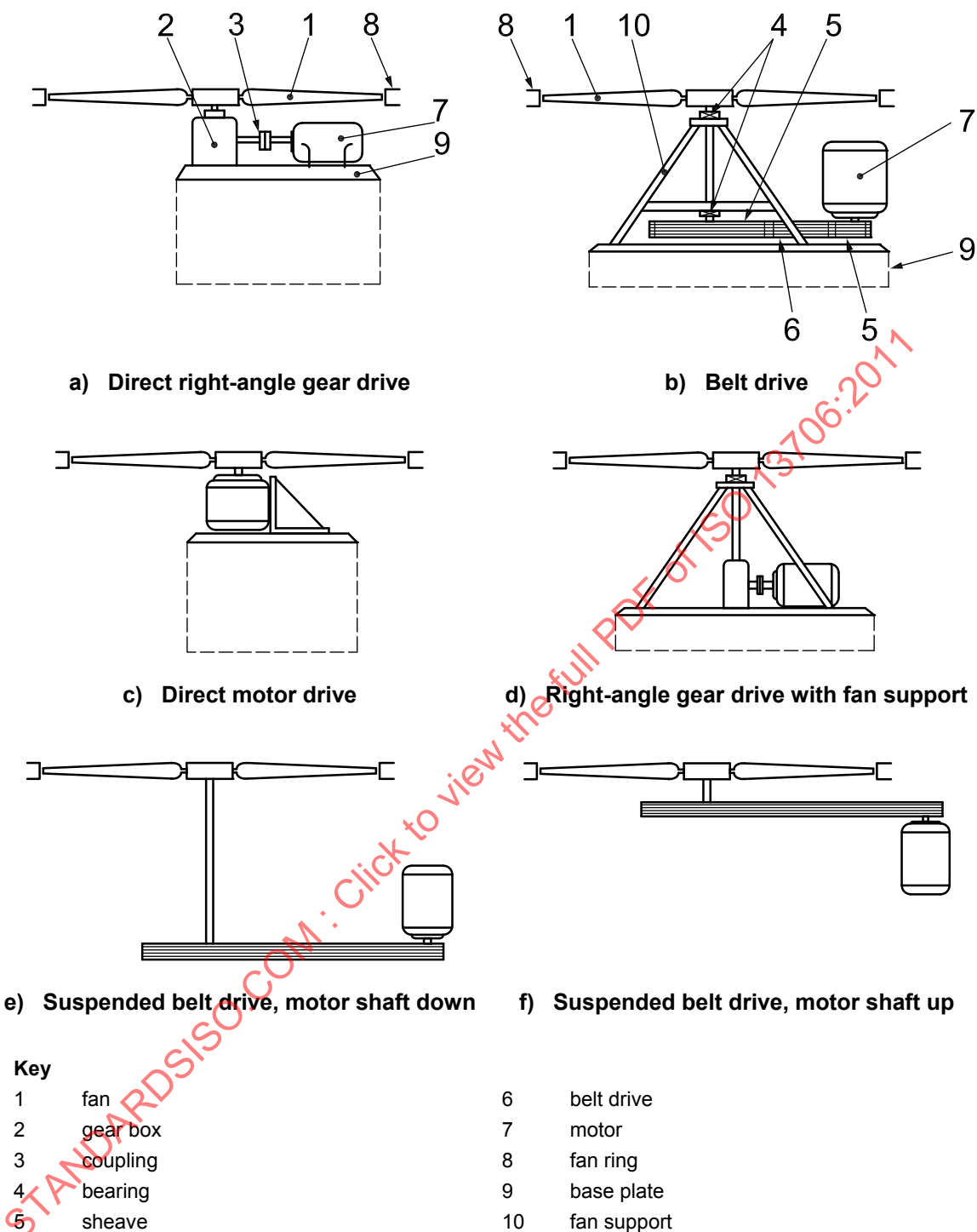
Figure 8 — Typical drive arrangements
