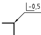
Figure 17 — State of edge common to all the edges of a part
