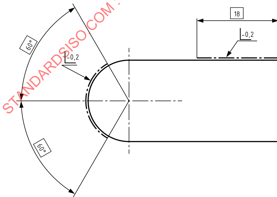
Figure 23 — Limited areas of an edge represented by long-dashed-dotted lines
