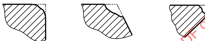
Figure 2 — Examples of undercut on an external edge
