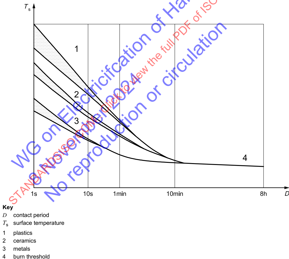
Figure 1 — Illustration of general relationship between burn threshold and contact period when hot surface is touched by skin
