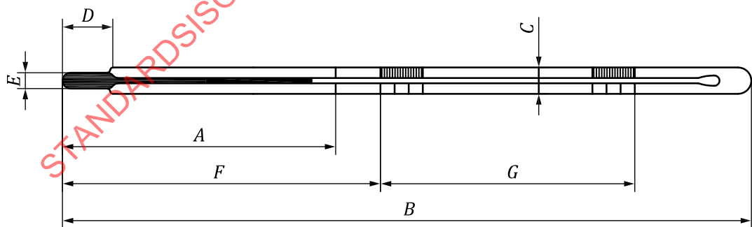
Figure C.2 — Low-temperature thermometer
