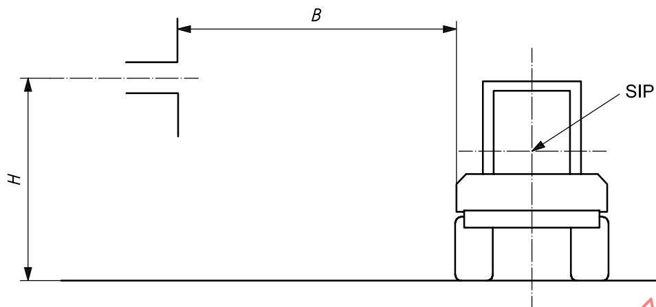
a) Dipole antenna in position to measure vertical component of radiation
