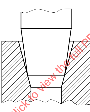
Case B — Valve taper less than cylinder — Acceptable, can be used
