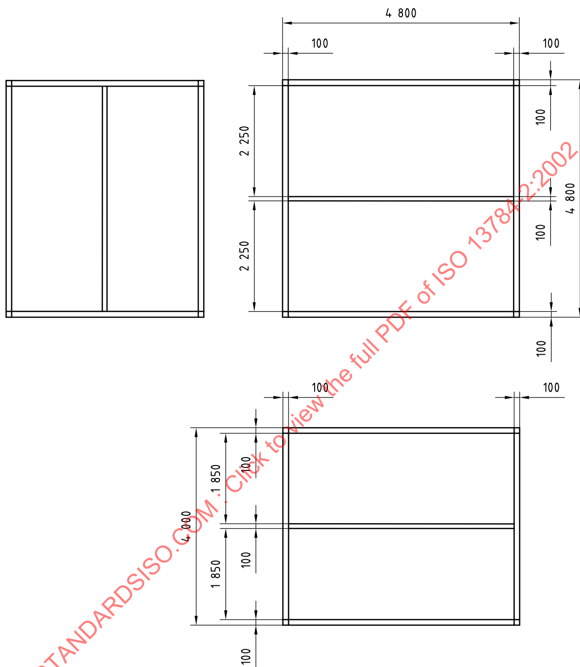
Figure 2 — Example of internal structural framework
