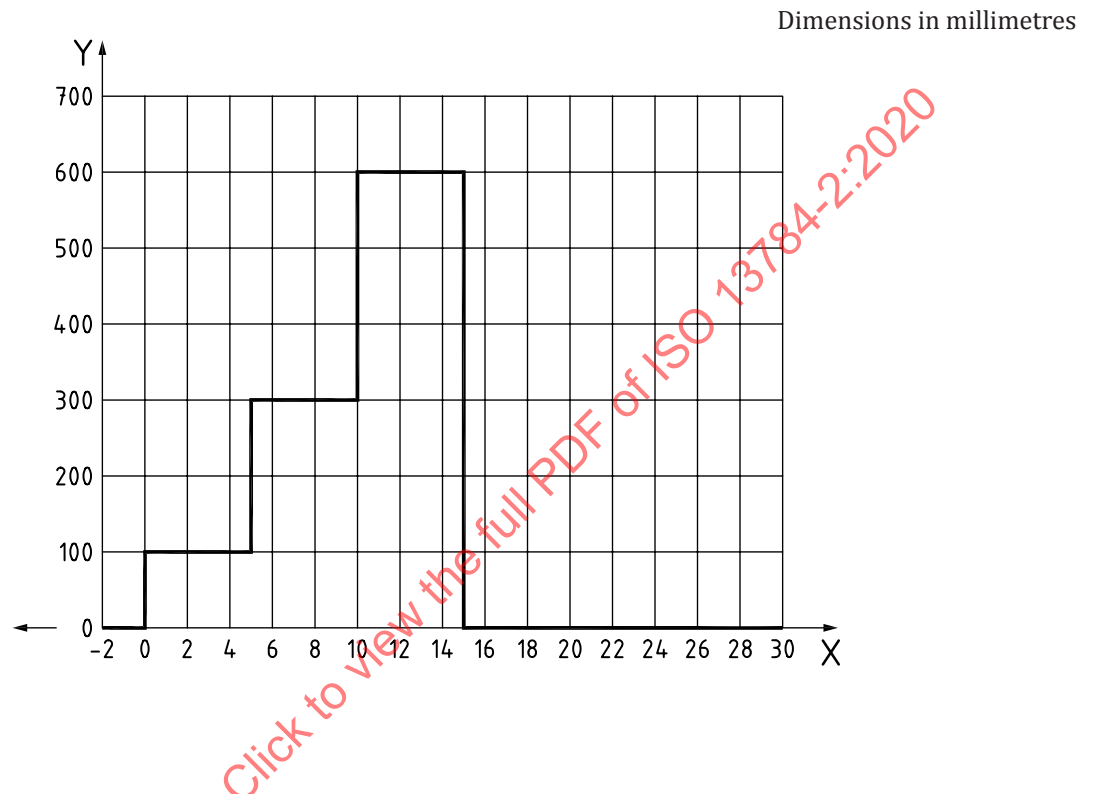
Figure 6 — Burner heat output programme (as described in 8.5 )
