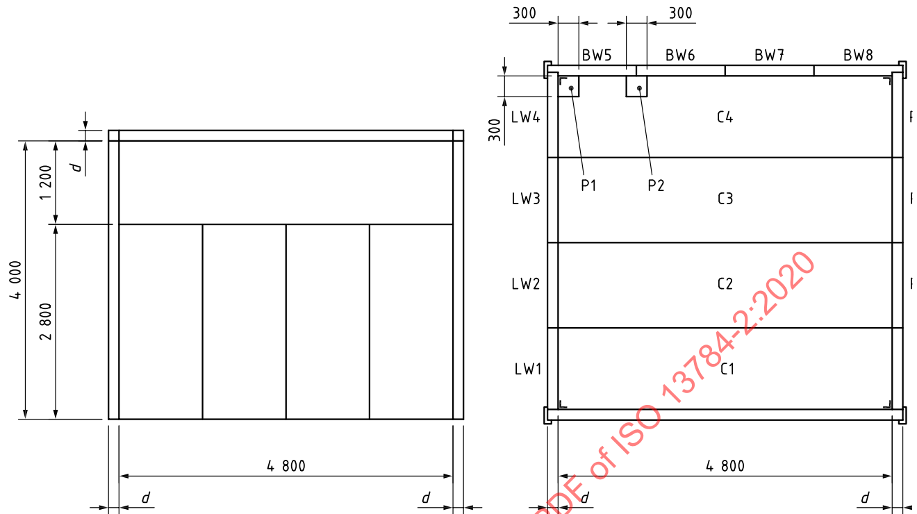
b) Plan showing alternative burner positions
