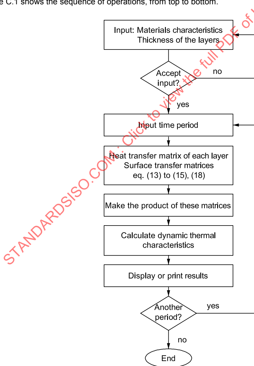
Figure C.1 — Flow chart of the calculation method
