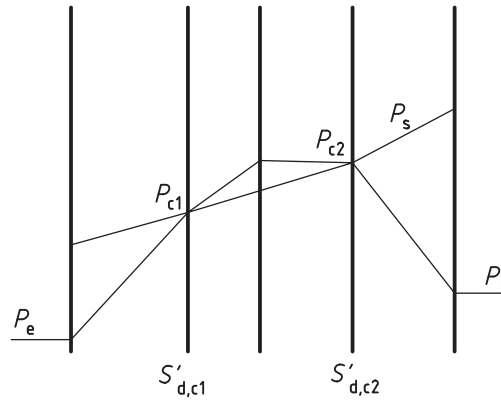
Figure 6 — Evaporation from a building component, when condensation has occurred in two interfaces
