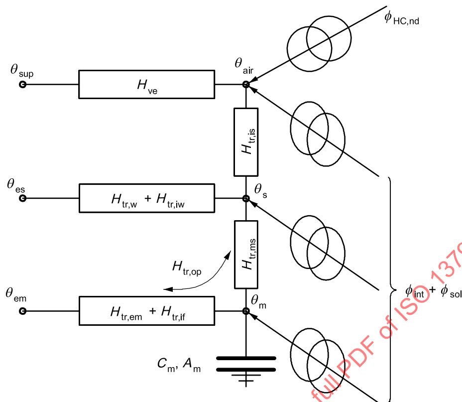
Figure B.1 — Modified RC network
