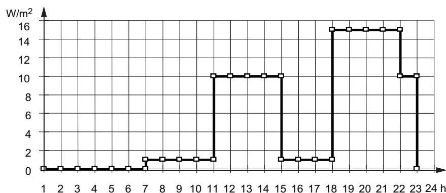
Figure 18 — Internal gains
