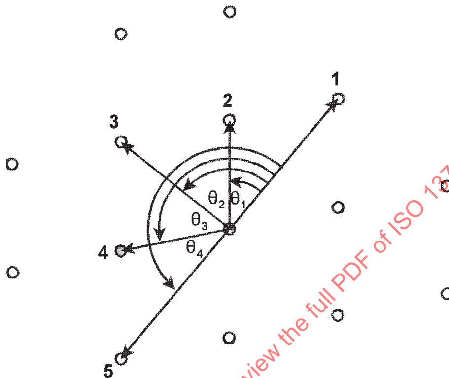
Figure E.1 — Example of measurement of zone-axis SAED patterns
