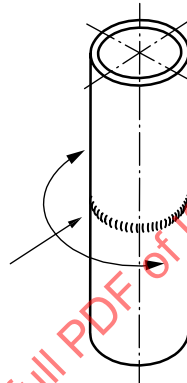
PG pipe : fixed axis : horizontal weld : vertical downward
