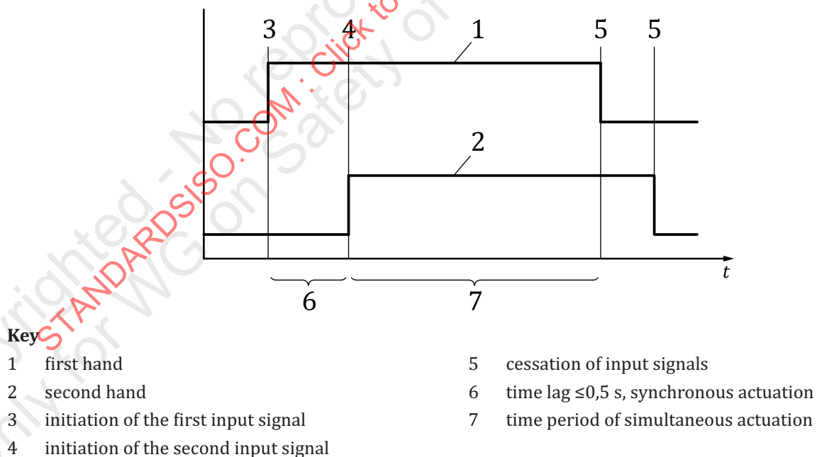
Figure 2 — Input signals in the case of synchronous actuation
