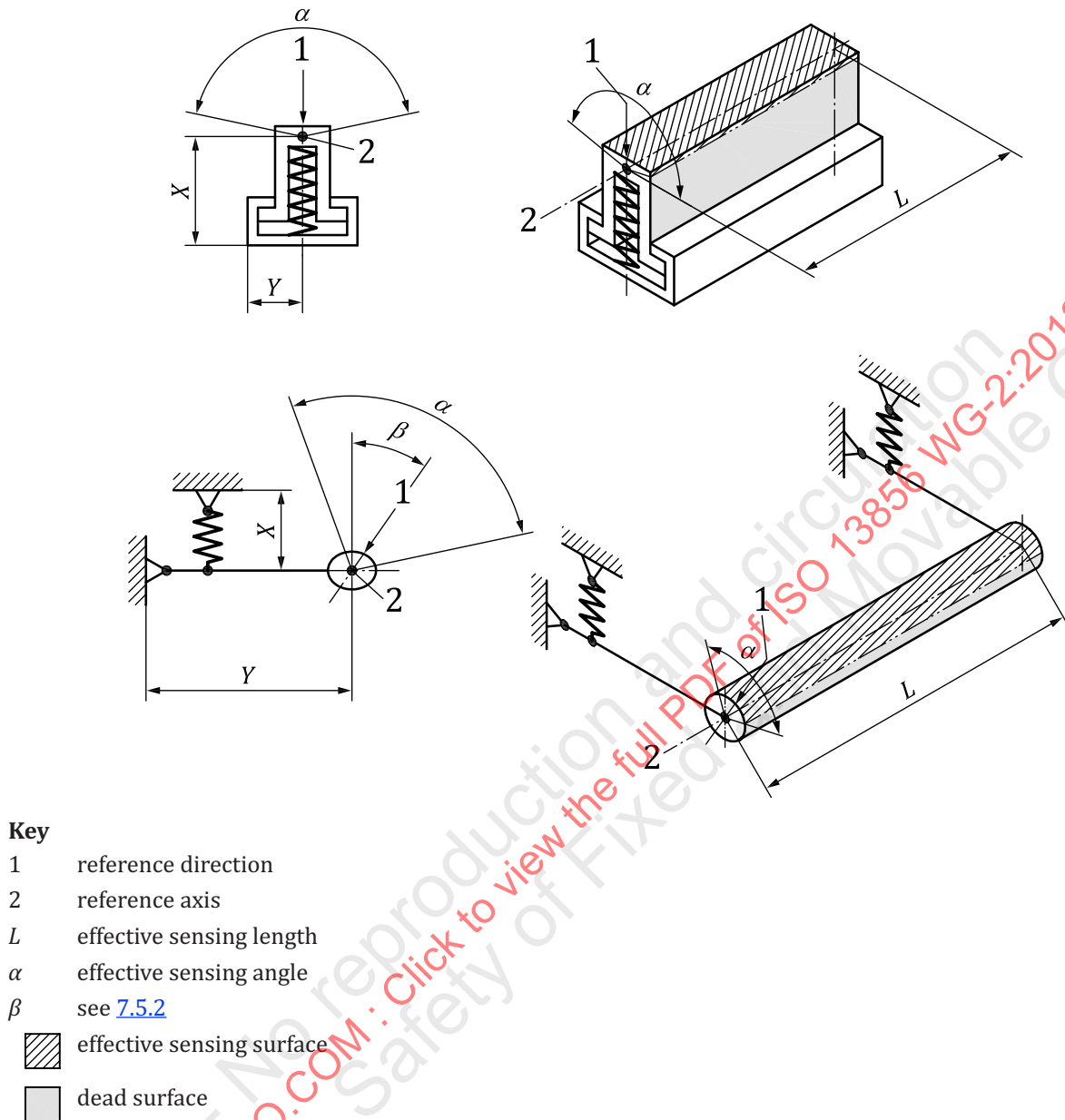
Figure 3 — Effective sensing surfaces of pressure-sensitive bars
