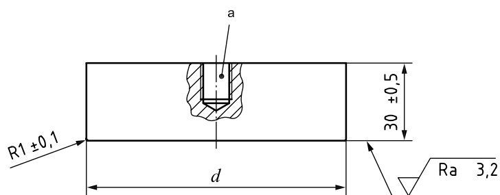
Test pieces 2, 3 and 4
